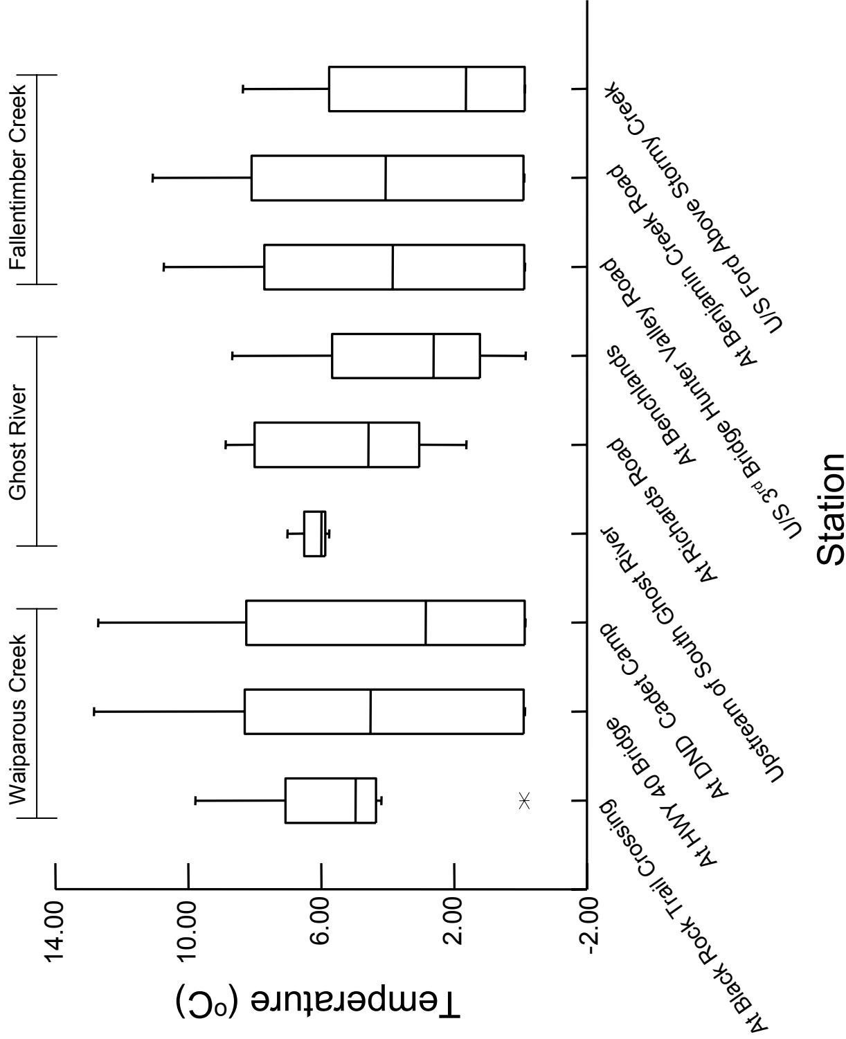
Figure 15.2 : Water Quality Monitoring Program 2004-2005 – Box Plots Temperature
