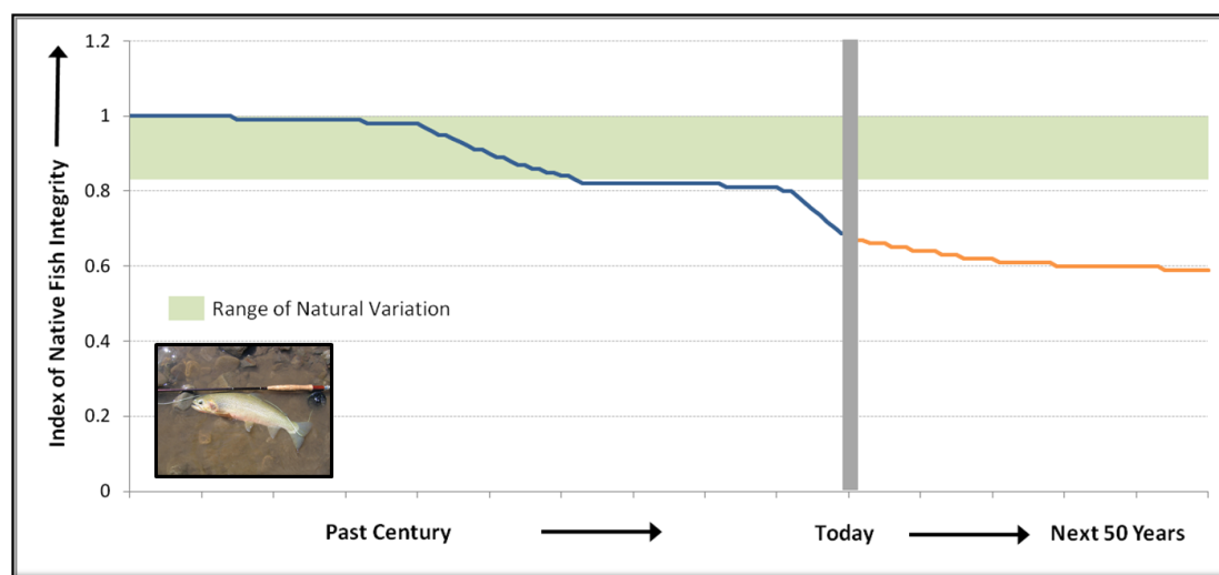
Figure 23. Projected changes in Index of Native Fish Integrity.
