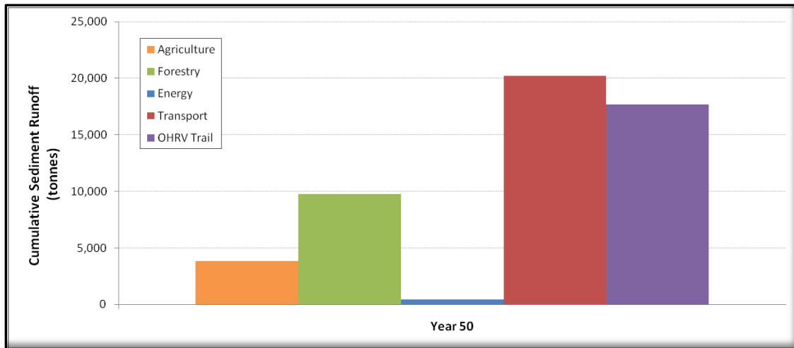
Figure 19. Relative land use sector contributions of sediment runoff.
