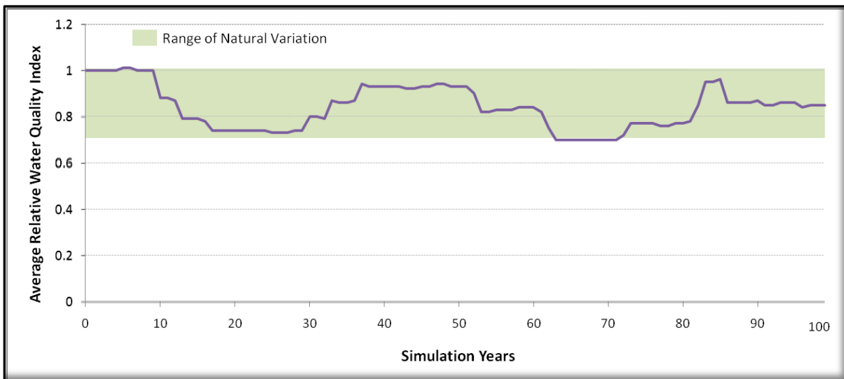
Figure 5. Natural year-to-year variability of relative water quality caused by inter-annual variation in precipitation and fire.
