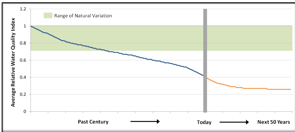
Figure 22. Change in relative river water quality index.
